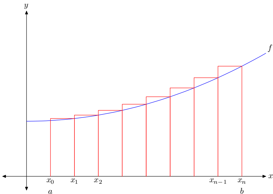
Figure 1 Using the right endpoint to calculate the height of each rectangle.
