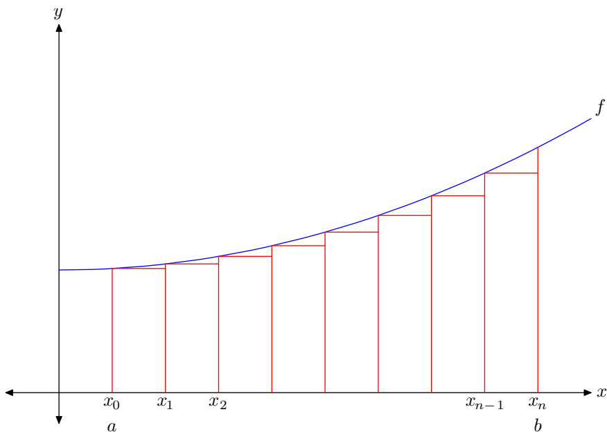
Figure 1 Using the left endpoint to calculate the height of each rectangle.
