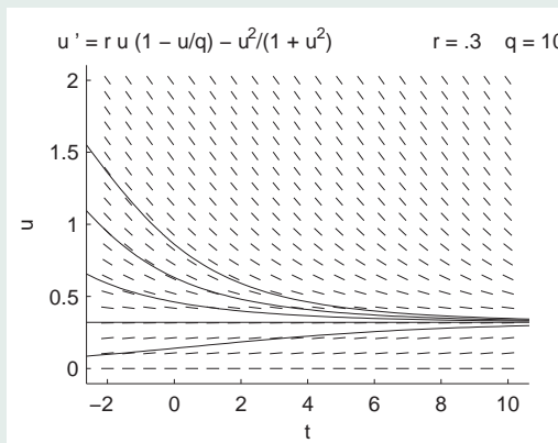
Figure 3: There is a stable equilibrium point at u_1 .
