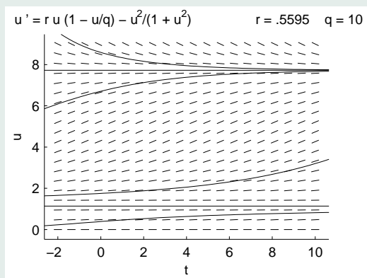
Figure 7: Increasing r u_1 and u_2 have coalesced into one semi stable equilibrium point.
