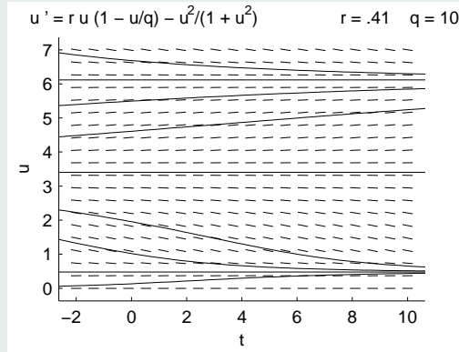
Figure 5: Stable equilibrium point at u_1 , unstable equilibrium point at u_2 , and a stable equilibrium point at u_3 .
