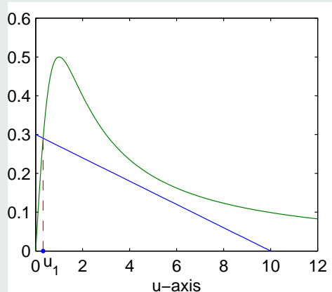
Figure 3: There is a stable equilibrium point at u_1 .
