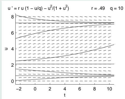
Figure 6: As r increases u_1 and u_2 move closer together.
